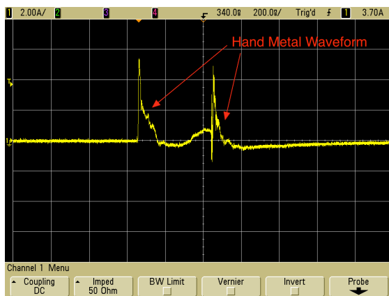
Figure 7. Secondary event showing human metal waveform characteristics. Scale factors: 2 A/div and 200 ns/div.
