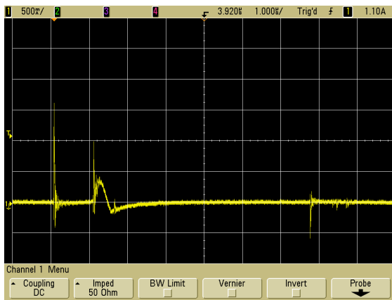
Figure 5. Long time view showing negative event. Scale factors: 500 mA/div and 1 \mu\text{s}/\text{div} .
